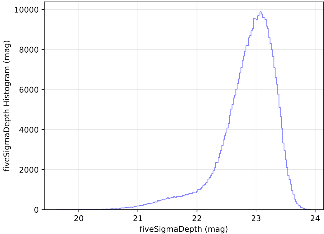
internal_u_expt60_nscale1.0v3.4_10yrs All sky z band: fiveSigmaDepth Histogram
