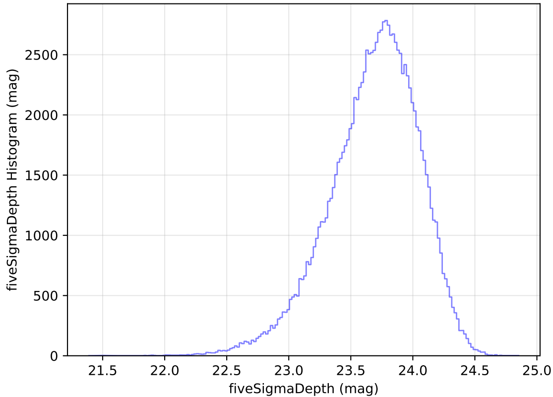
internal_u_expt60_nscale1.0v3.4_10yrs All sky u band: fiveSigmaDepth Histogram
