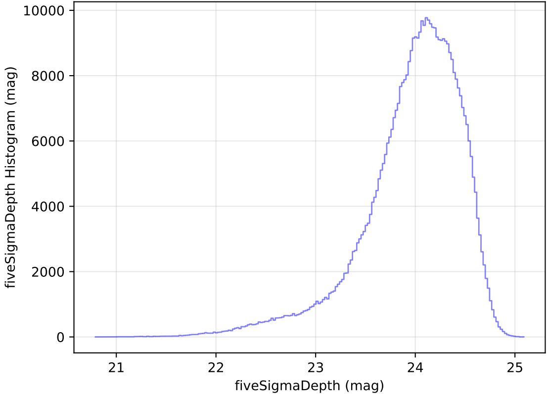
internal_u_expt60_nscale1.0v3.4_10yrs All sky r band: fiveSigmaDepth Histogram
