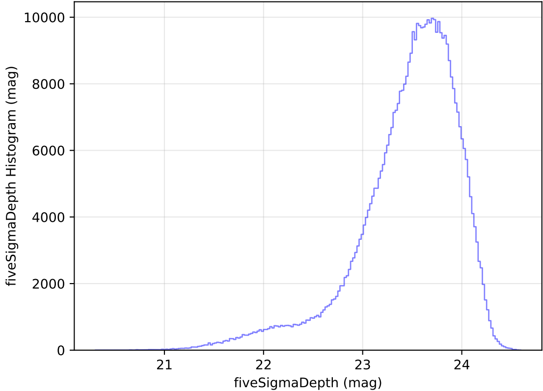
internal_u_expt60_nscale1.0v3.4_10yrs All sky i band: fiveSigmaDepth Histogram
