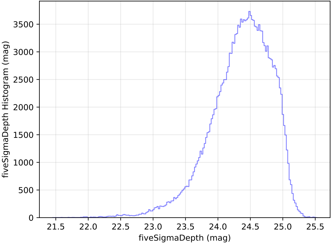
internal_u_expt60_nscale1.0v3.4_10yrs All sky g band: fiveSigmaDepth Histogram
