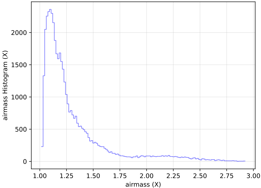
internal_u_expt60_nscale1.0v3.4_10yrs Yr 1 z band: airmass Histogram
