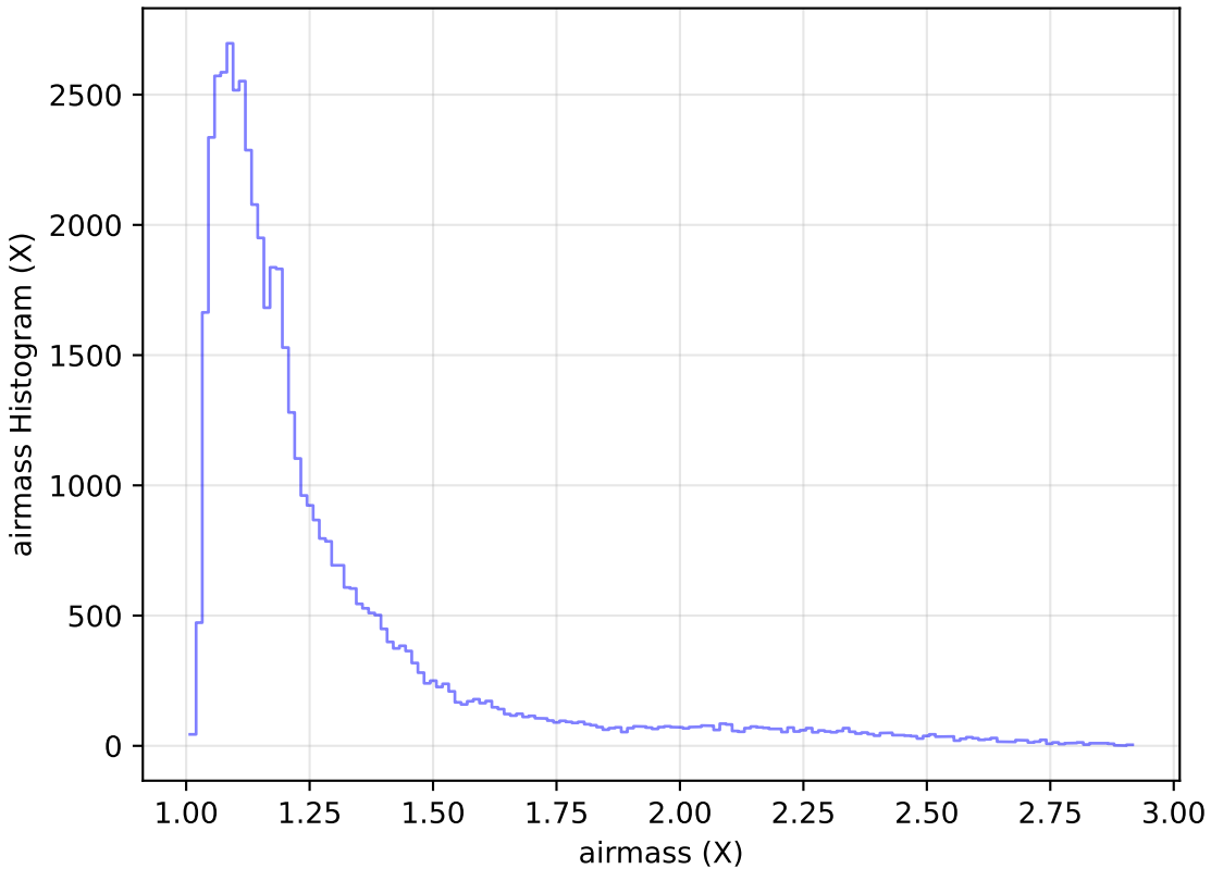
internal_u_expt60_nscale1.0v3.4_10yrs Yr 1 i band: airmass Histogram
