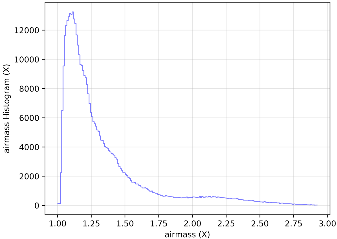
internal_u_expt60_nscale1.0v3.4_10yrs WFD z band: airmass Histogram
