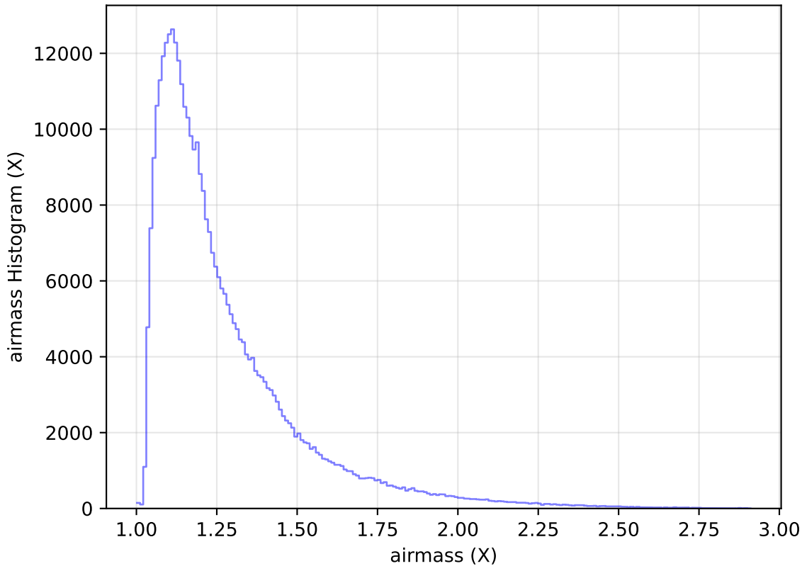
internal_u_expt60_nscale1.0v3.4_10yrs WFD y band: airmass Histogram
