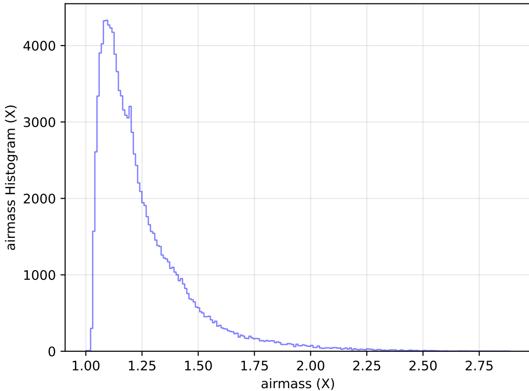
internal_u_expt60_nscale1.0v3.4_10yrs WFD u band: airmass Histogram
