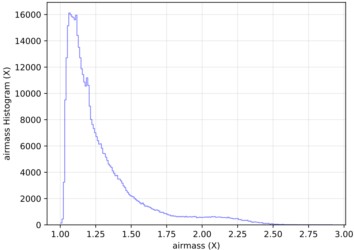
internal_u_expt60_nscale1.0v3.4_10yrs WFD r band: airmass Histogram
