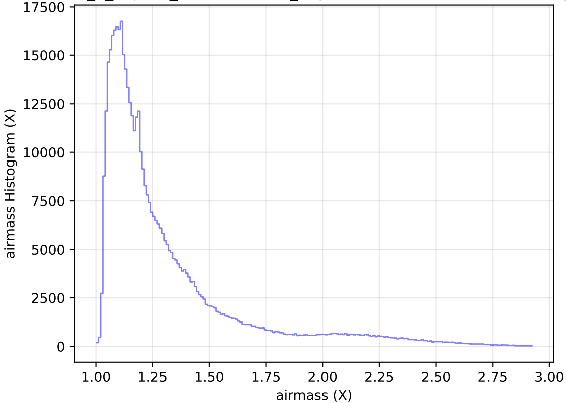
internal_u_expt60_nscale1.0v3.4_10yrs WFD i band: airmass Histogram
