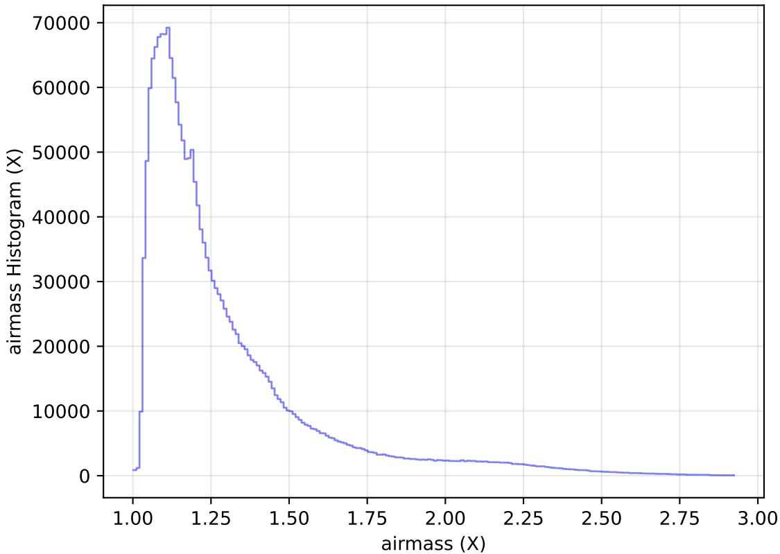
internal_u_expt60_nscale1.0v3.4_10yrs WFD all bands: airmass Histogram
