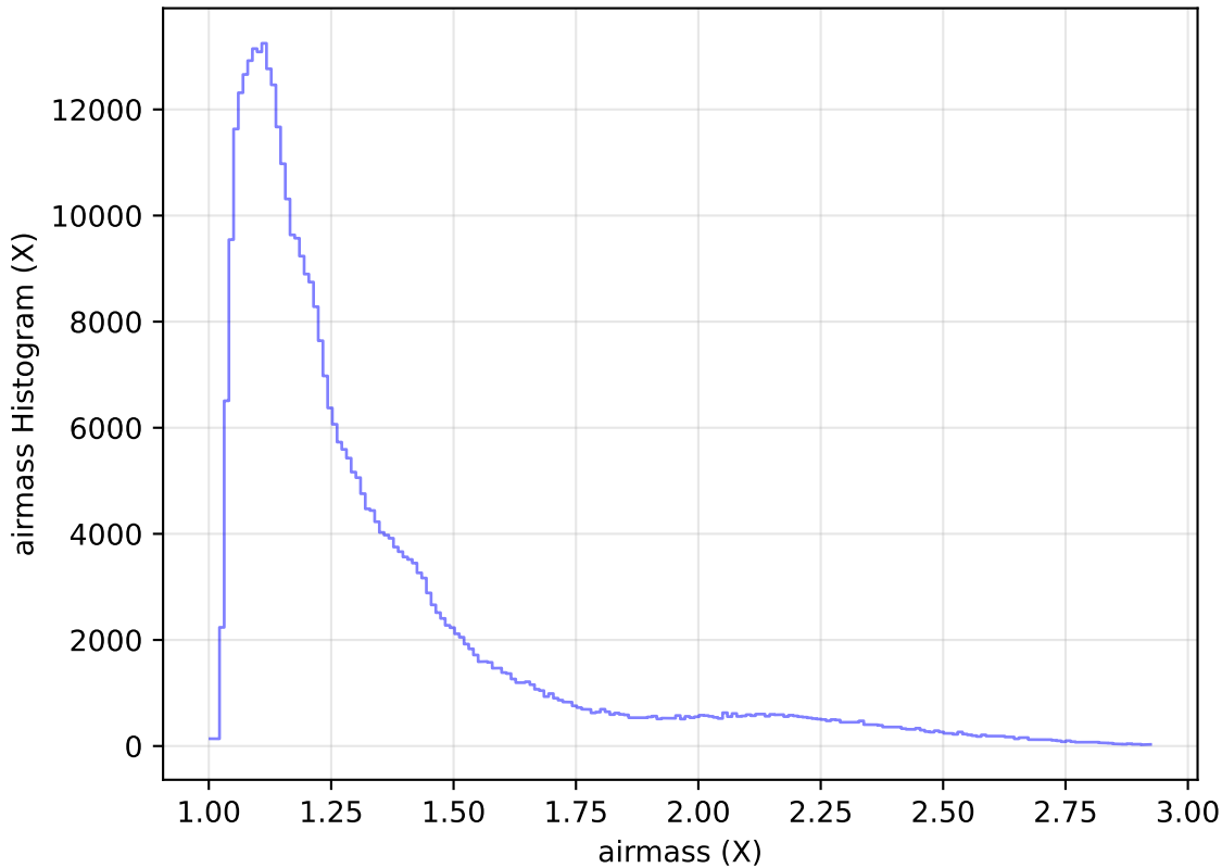
internal_u_expt60_nscale1.0v3.4_10yrs All sky z band: airmass Histogram
