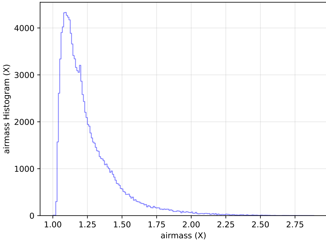
internal_u_expt60_nscale1.0v3.4_10yrs All sky u band: airmass Histogram
