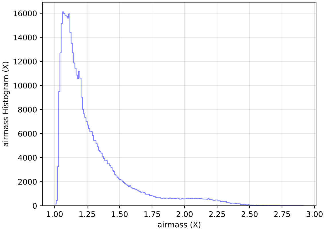
internal_u_expt60_nscale1.0v3.4_10yrs All sky r band: airmass Histogram
