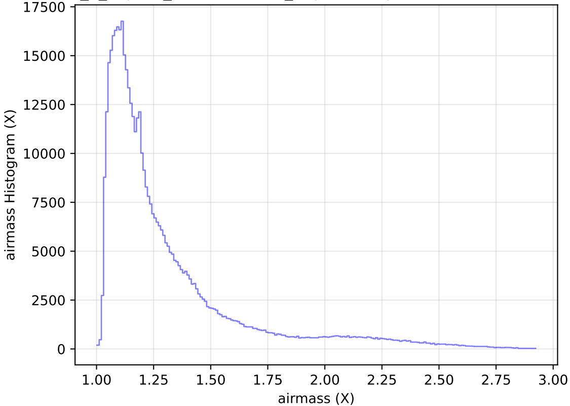
internal_u_expt60_nscale1.0v3.4_10yrs All sky i band: airmass Histogram
