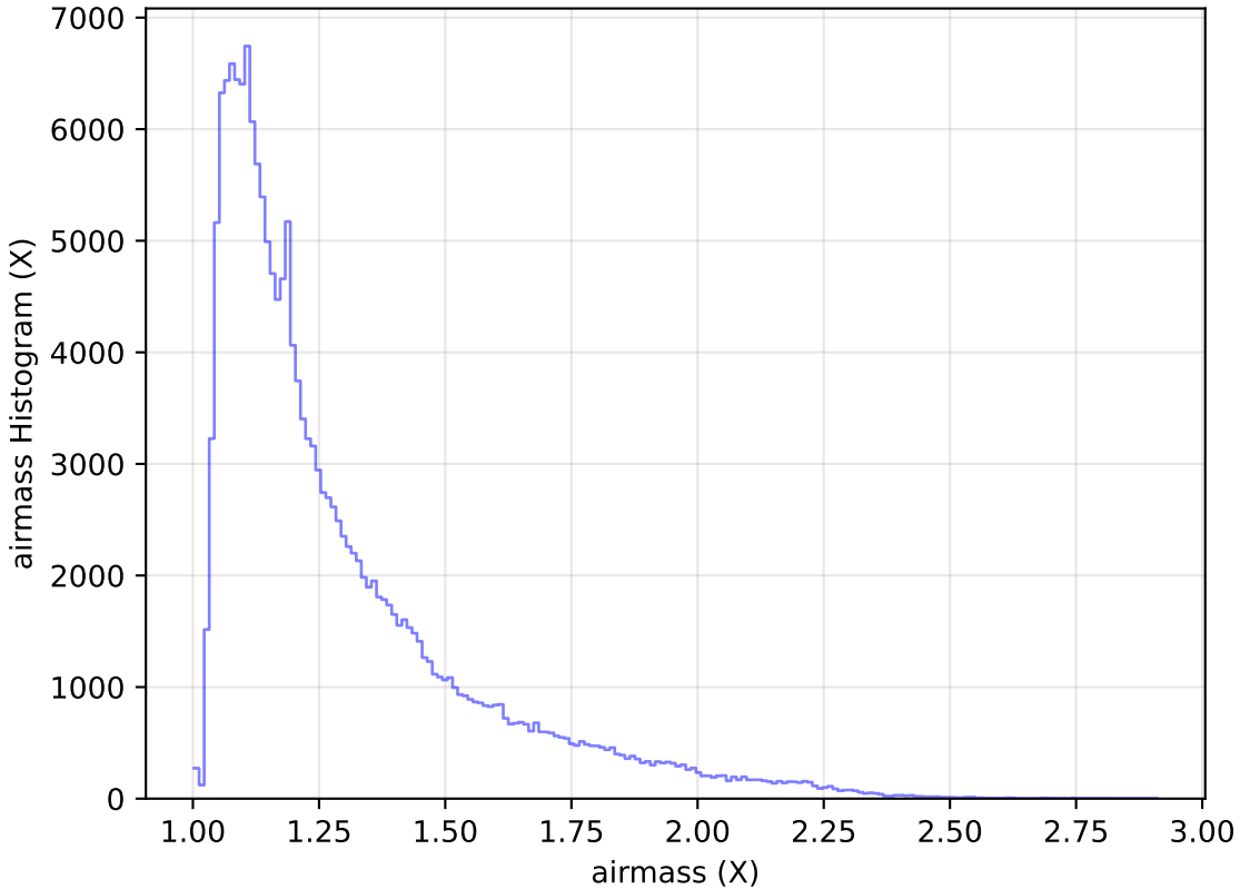
internal_u_expt60_nscale1.0v3.4_10yrs All sky g band: airmass Histogram
