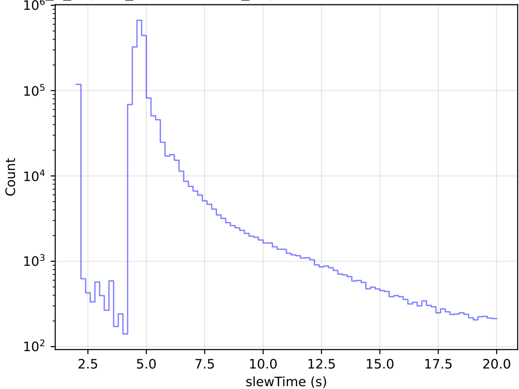
internal_u_expt60_nscale1.0v3.4_10yrs All visits: Zoom Slew Time Histogram
