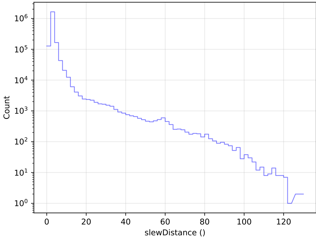
internal_u_expt60_nscale1.0v3.4_10yrs All visits: Slew Distance Histogram
