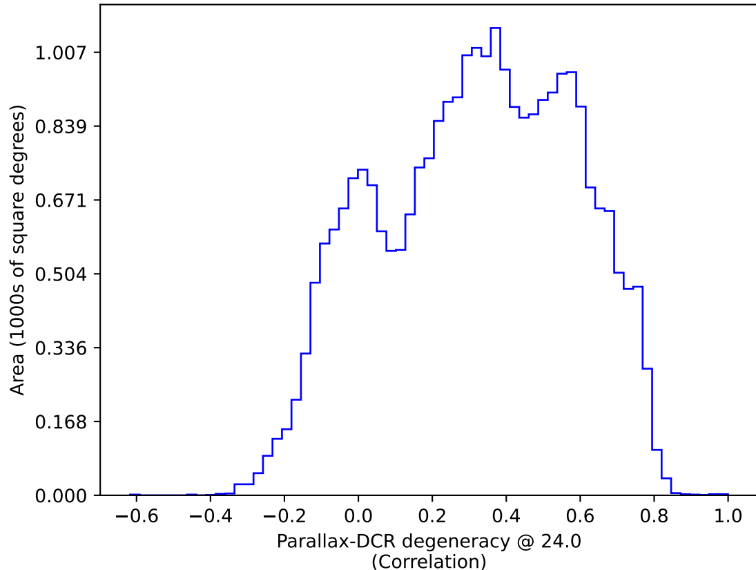
internal_u_expt60_nscale1.0v3.4_10yrs All sky: Parallax-DCR degeneracy @ 24.0
