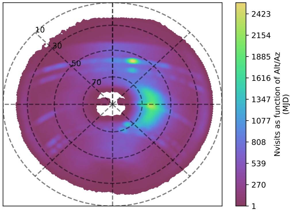
internal_u_expt60_nscale1.0v3.4_10yrs z band: Nvisits as function of Alt/Az
