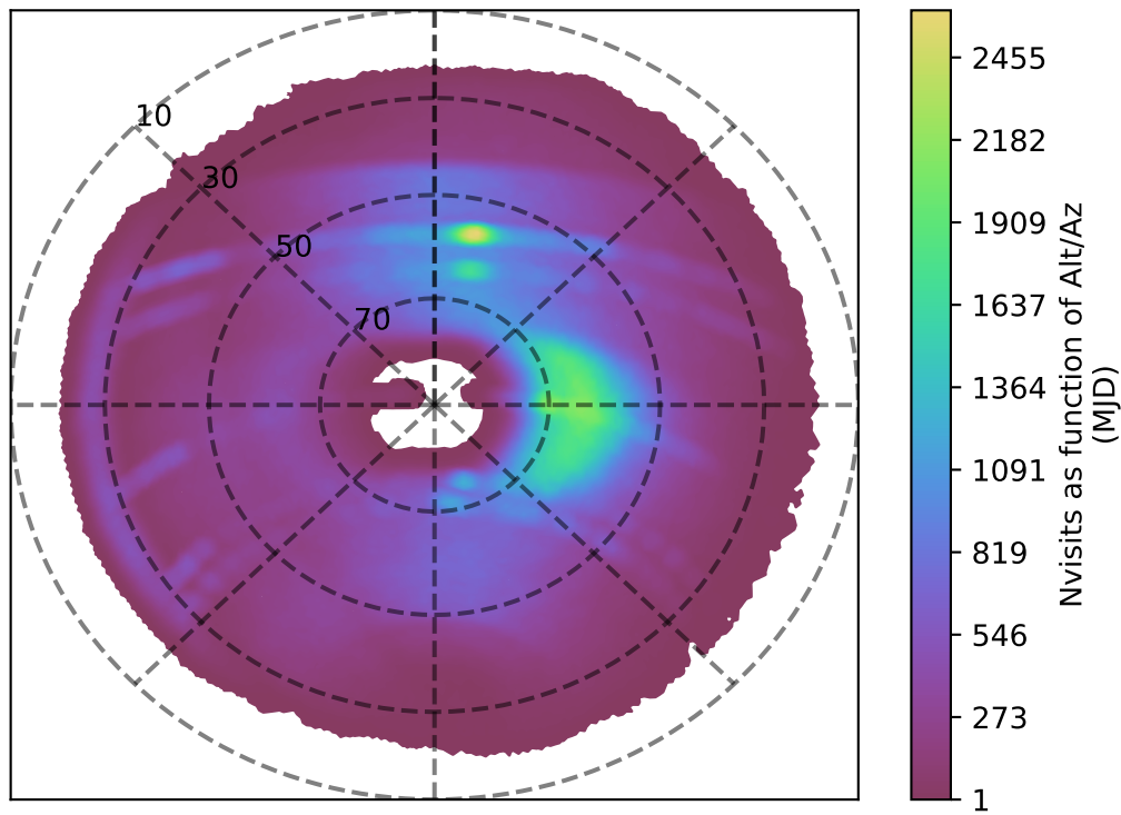
internal_u_expt60_nscale1.0v3.4_10yrs r band: Nvisits as function of Alt/Az
