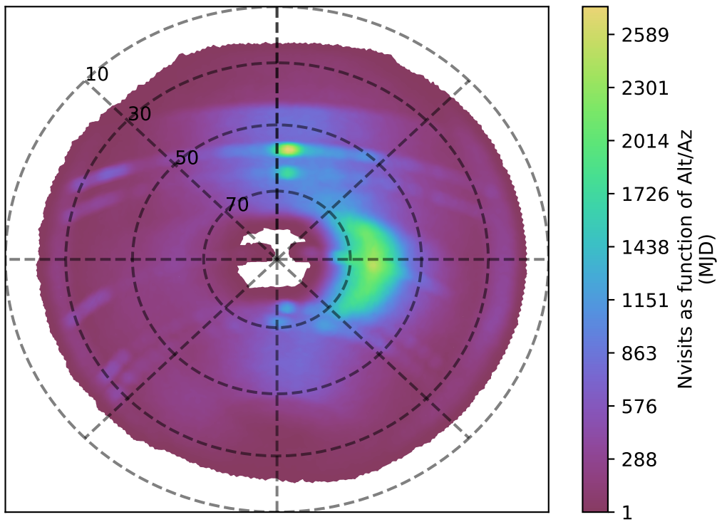
internal_u_expt60_nscale1.0v3.4_10yrs i band: Nvisits as function of Alt/Az
