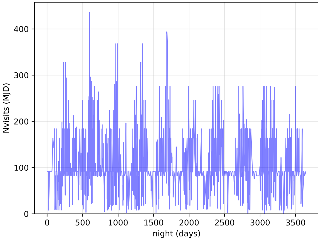
internal_u_expt60_nscale1.0v3.4_10yrs DDF: Nvisits
