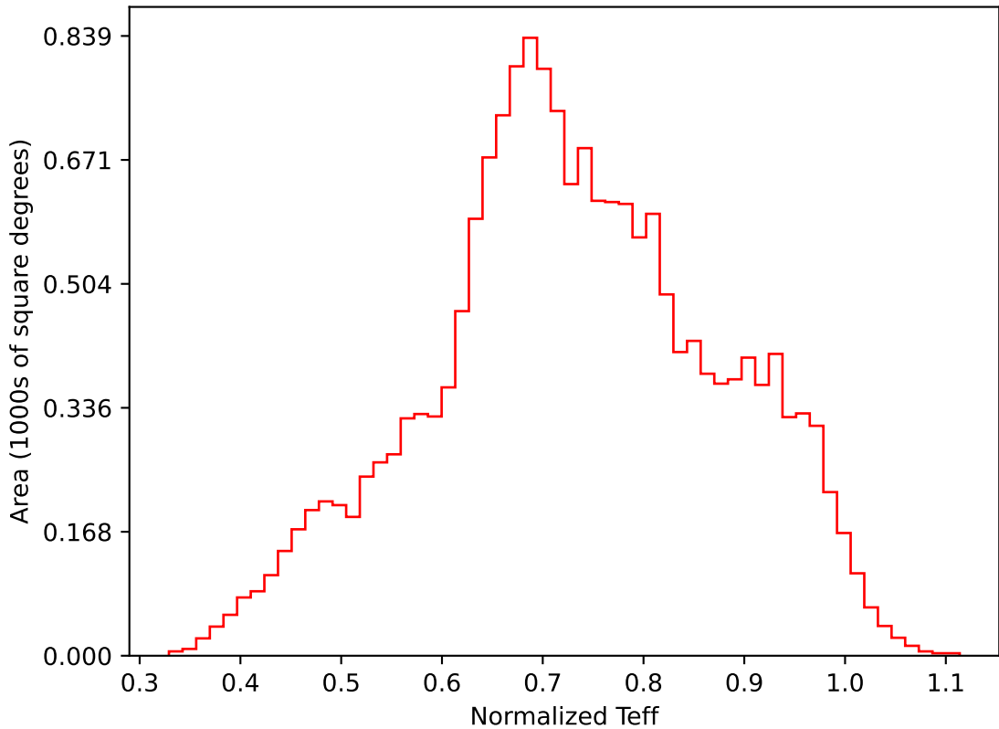
internal_u_expt60_nscale1.0v3.4_10yrs WFD i band: Normalized Teff
