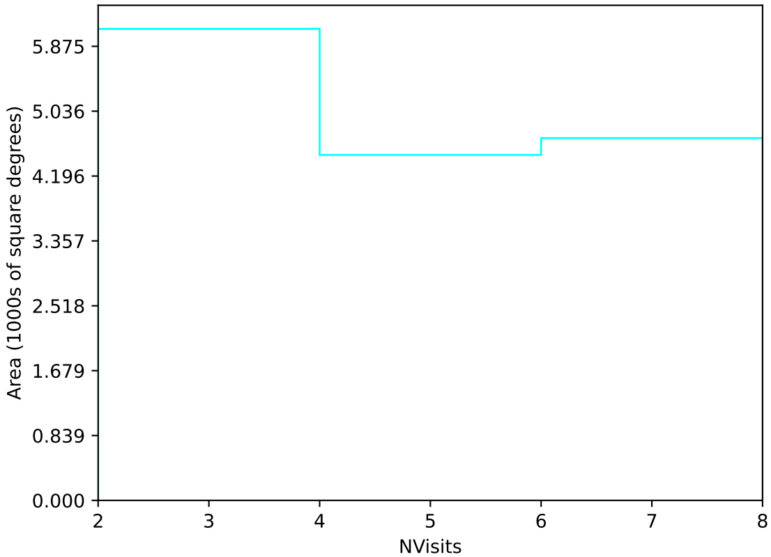
internal_u_expt60_nscale1.0v3.4_10yrs Yr 3-4 u band: NVisits
