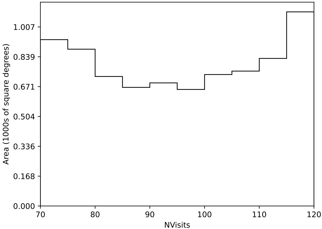
internal_u_expt60_nscale1.0v3.4_10yrs Yr 3-4 all bands: NVisits
