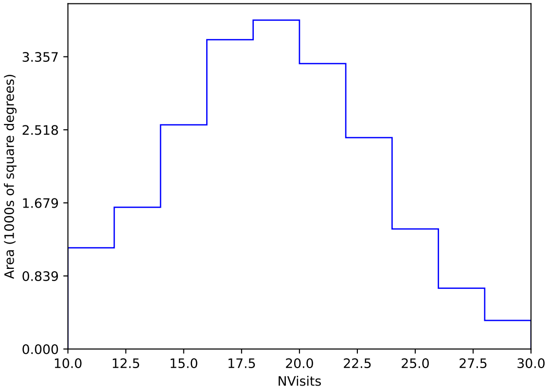
internal_u_expt60_nscale1.0v3.4_10yrs Yr 1 y band: NVisits
