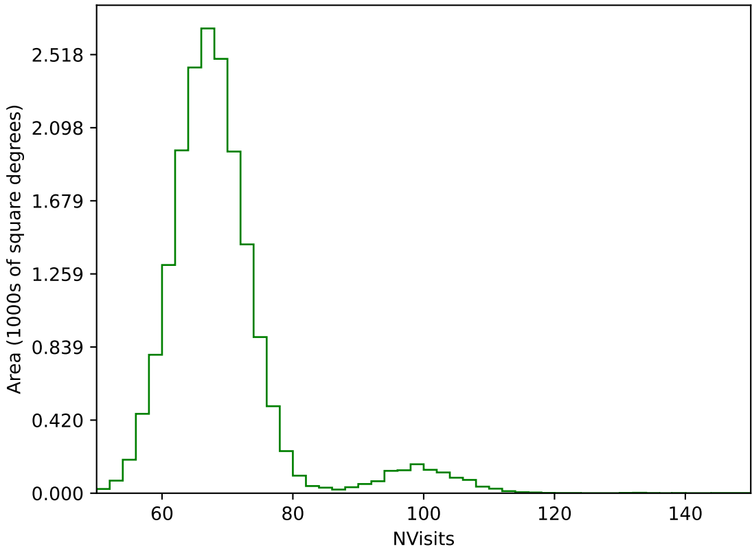
internal_u_expt60_nscale1.0v3.4_10yrs WFD g band: NVisits
