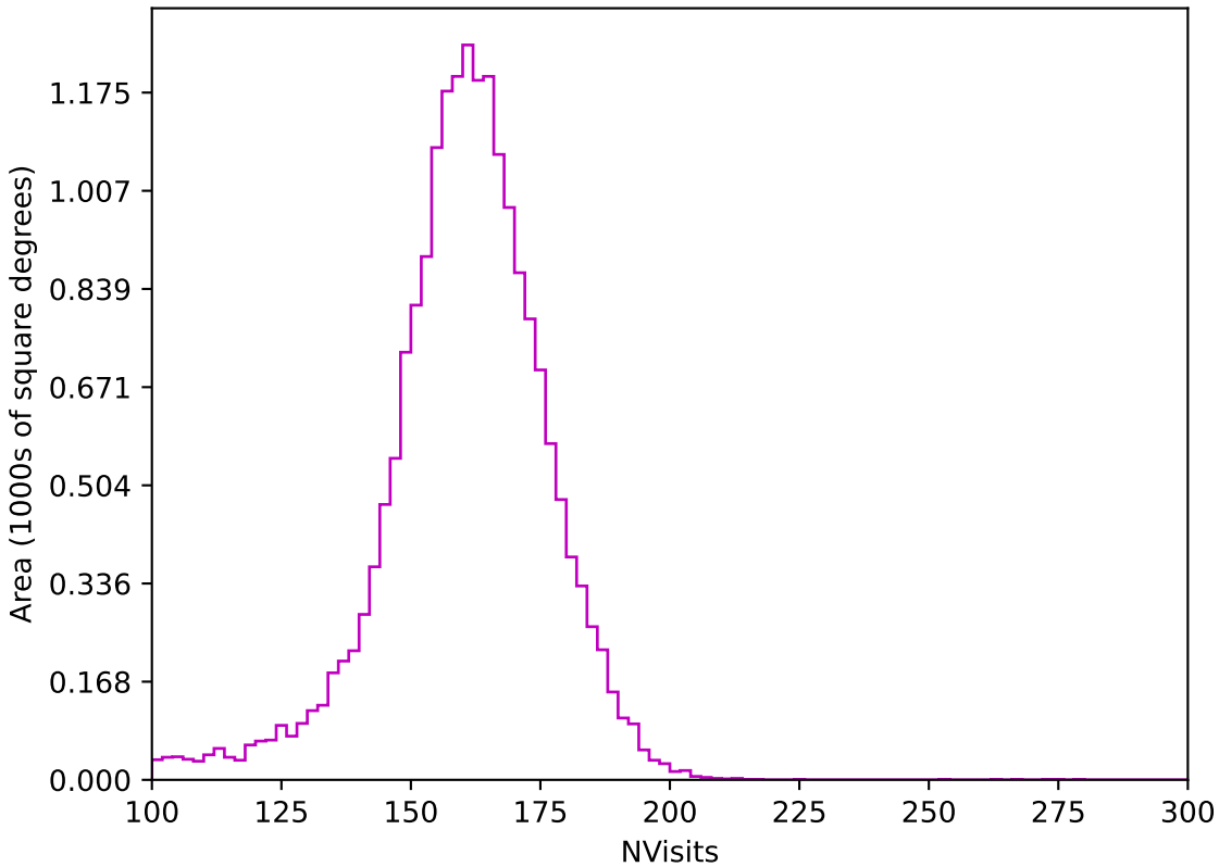
internal_u_expt60_nscale1.0v3.4_10yrs All sky z band: NVisits
