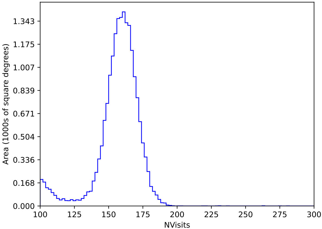
internal_u_expt60_nscale1.0v3.4_10yrs All sky y band: NVisits
