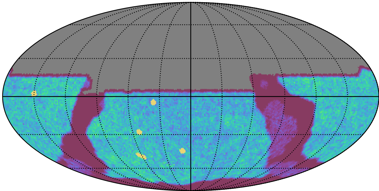
internal_u_expt60_nscale1.0v3.4_10yrs All sky u band: NVisits
