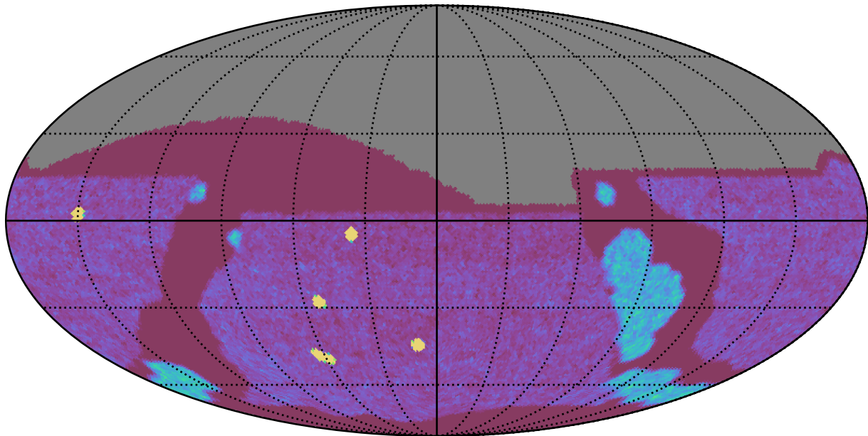
internal_u_expt60_nscale1.0v3.4_10yrs All sky g band: NVisits
