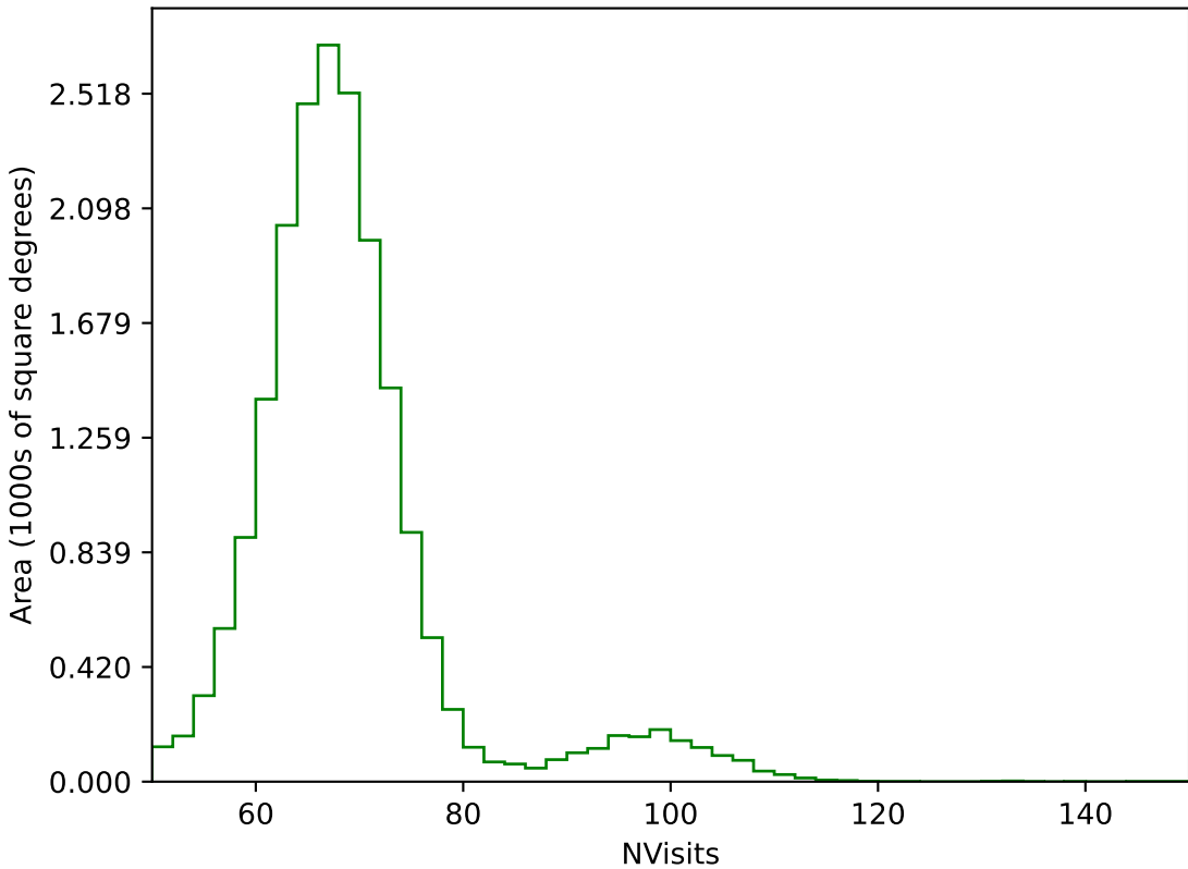
internal_u_expt60_nscale1.0v3.4_10yrs All sky g band: NVisits
