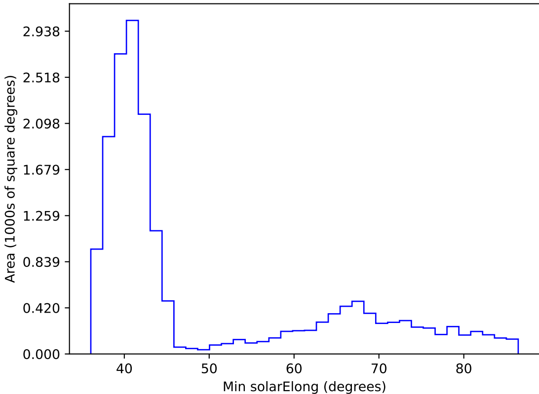
internal_u_expt60_nscale1.0v3.4_10yrs WFD i band: Min solarElong
