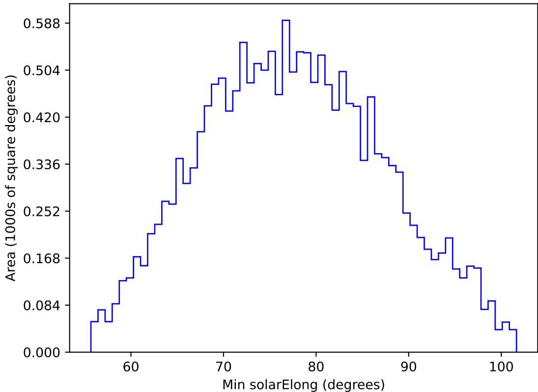
internal_u_expt60_nscale1.0v3.4_10yrs WFD g band: Min solarElong
