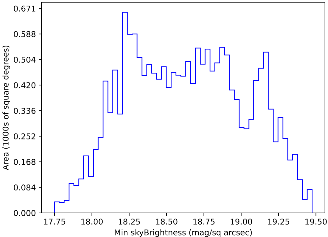
internal_u_expt60_nscale1.0v3.4_10yrs WFD r band: Min skyBrightness
