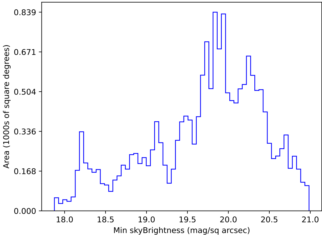
internal_u_expt60_nscale1.0v3.4_10yrs WFD g band: Min skyBrightness
