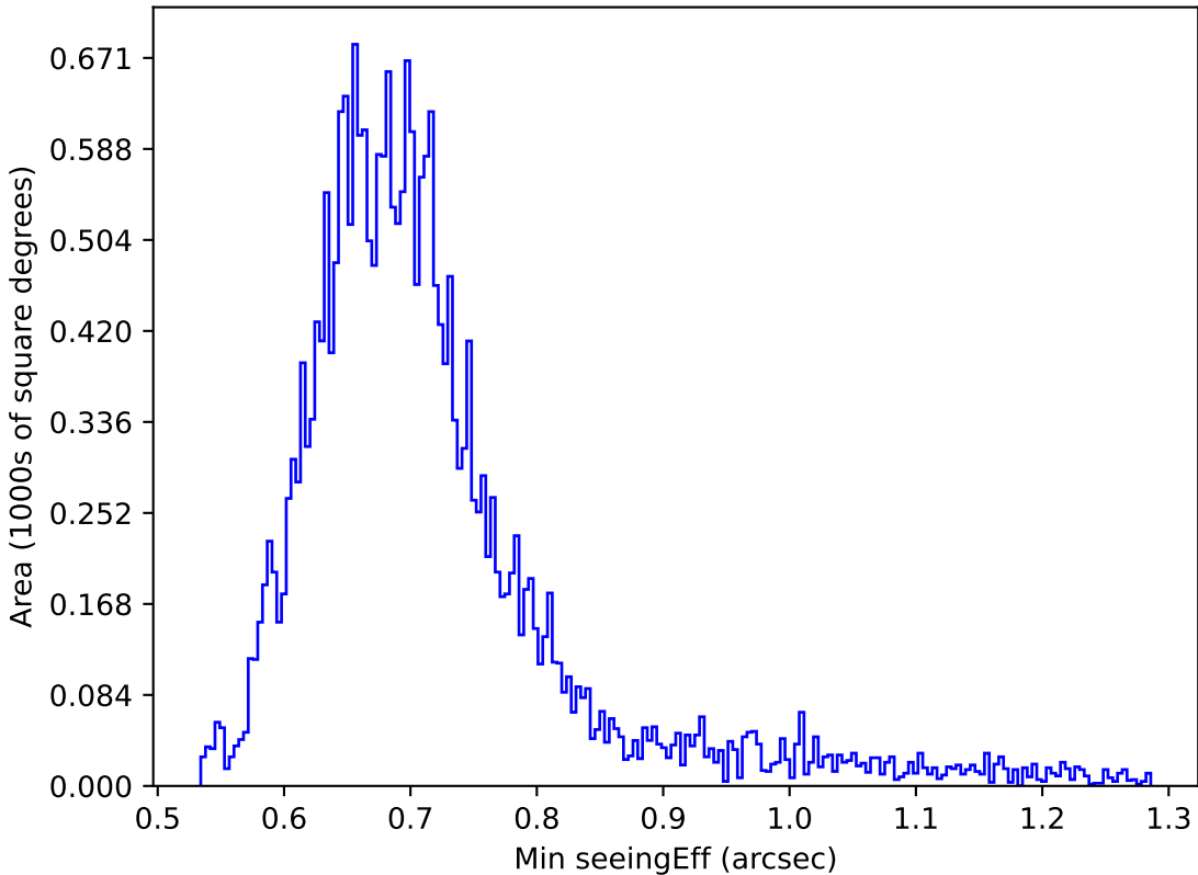
internal_u_expt60_nscale1.0v3.4_10yrs Yr 1 r band: Min seeingEff
