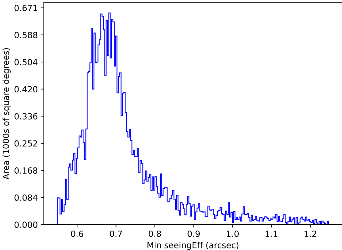
internal_u_expt60_nscale1.0v3.4_10yrs Yr 1 i band: Min seeingEff
