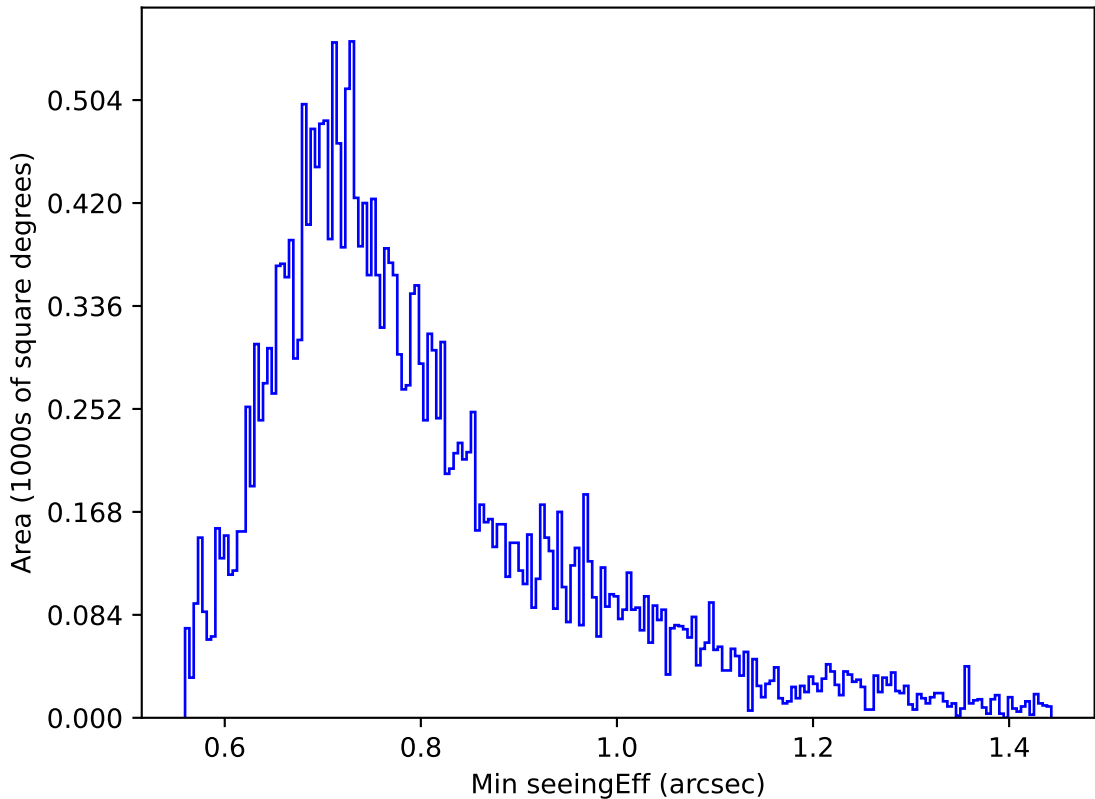
internal_u_expt60_nscale1.0v3.4_10yrs Yr 1 g band: Min seeingEff
