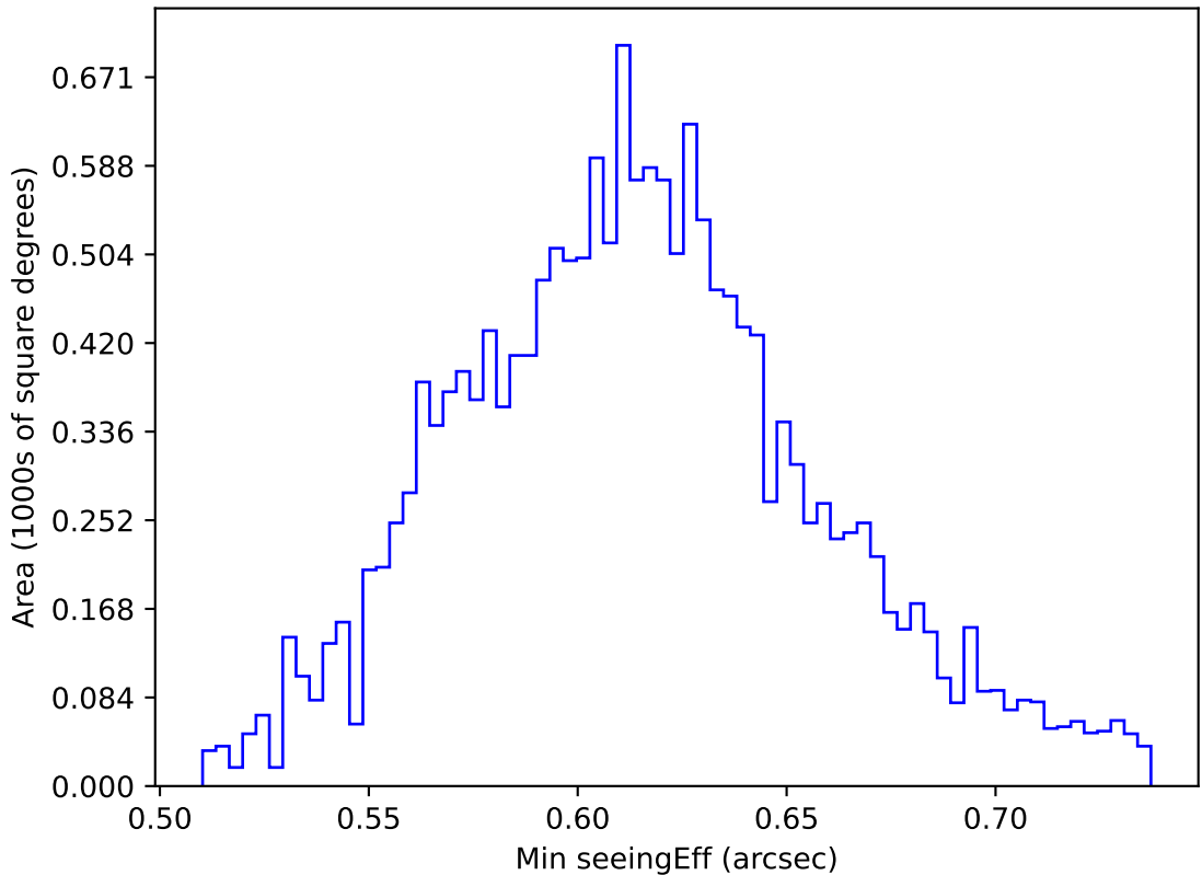
internal_u_expt60_nscale1.0v3.4_10yrs WFD z band: Min seeingEff
