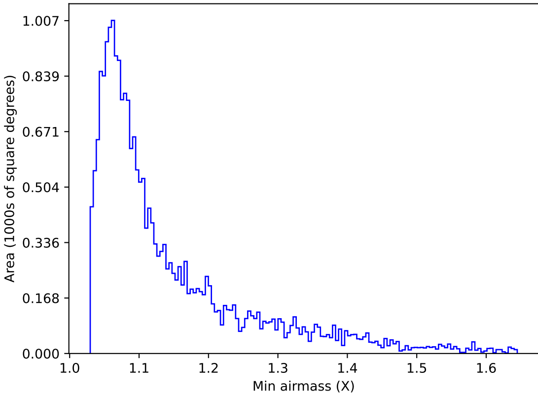
internal_u_expt60_nscale1.0v3.4_10yrs Yr 1 u band: Min airmass
