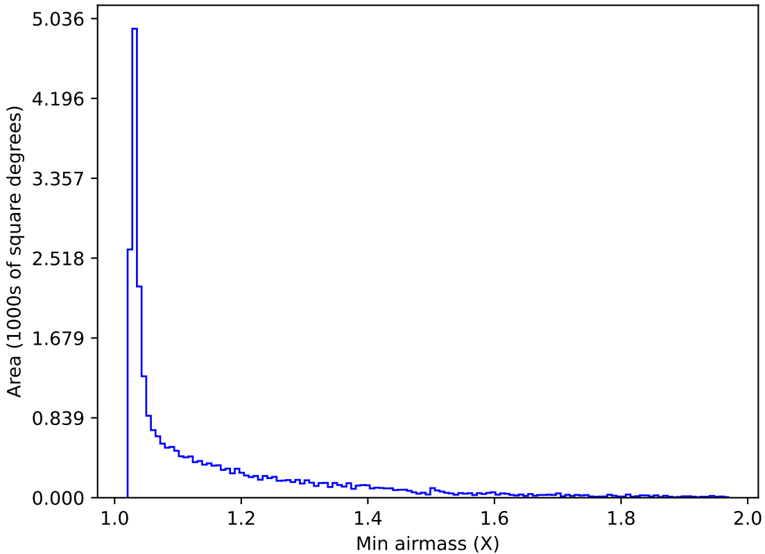
internal_u_expt60_nscale1.0v3.4_10yrs Yr 1 all bands: Min airmass
