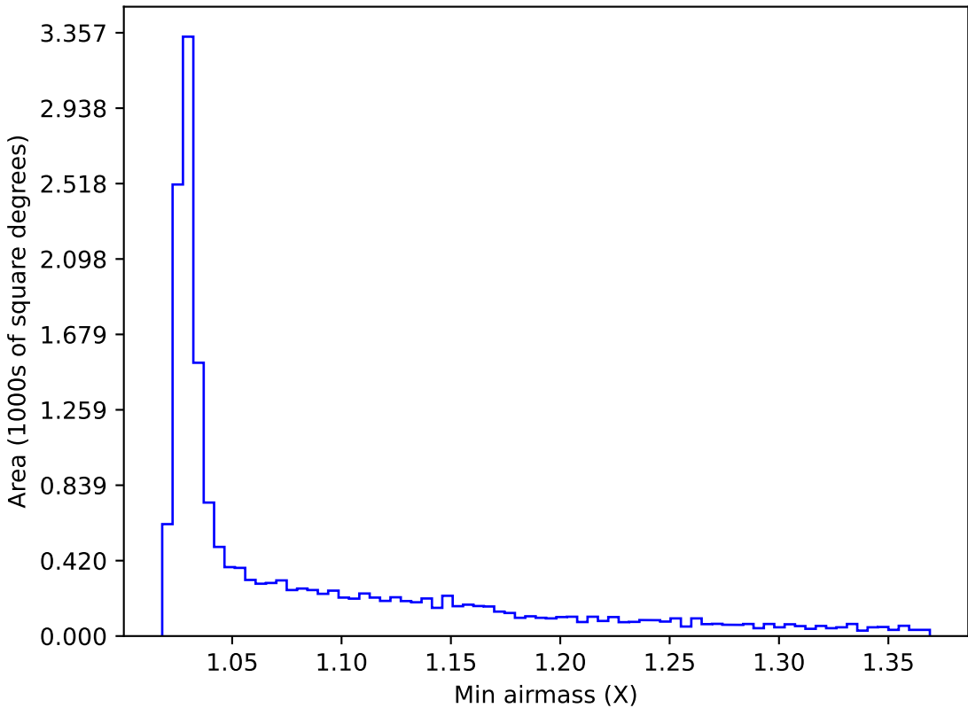
internal_u_expt60_nscale1.0v3.4_10yrs WFD z band: Min airmass
