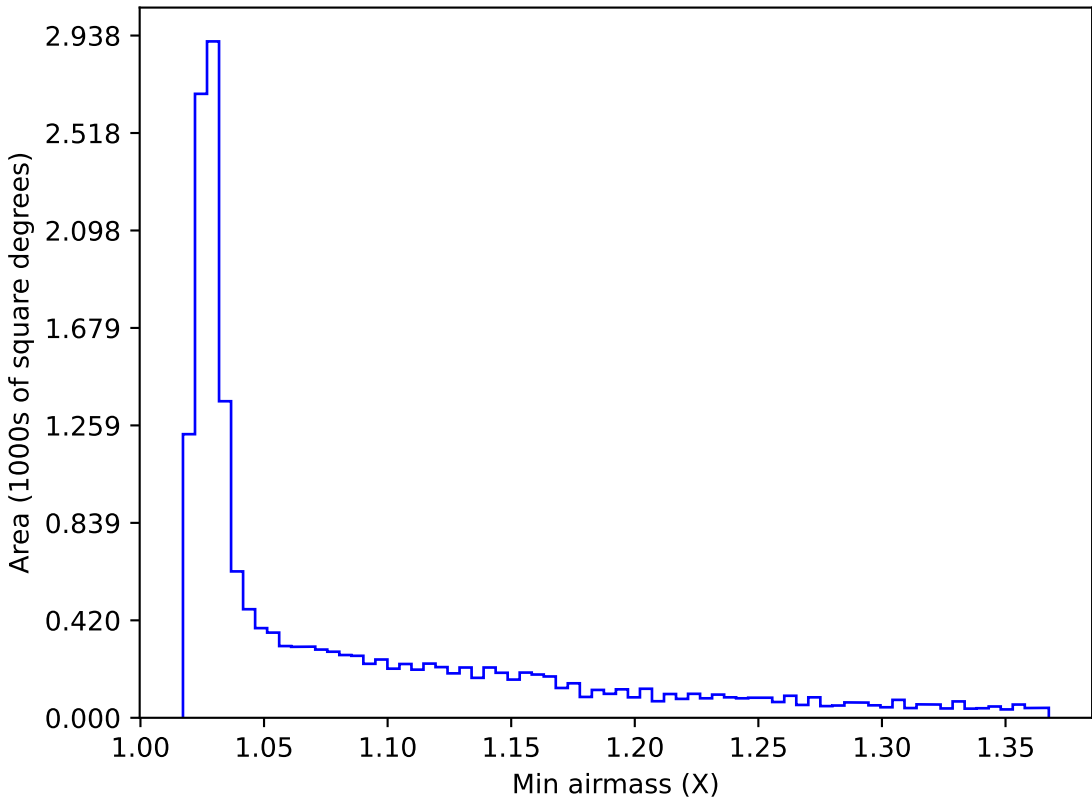
internal_u_expt60_nscale1.0v3.4_10yrs WFD r band: Min airmass
