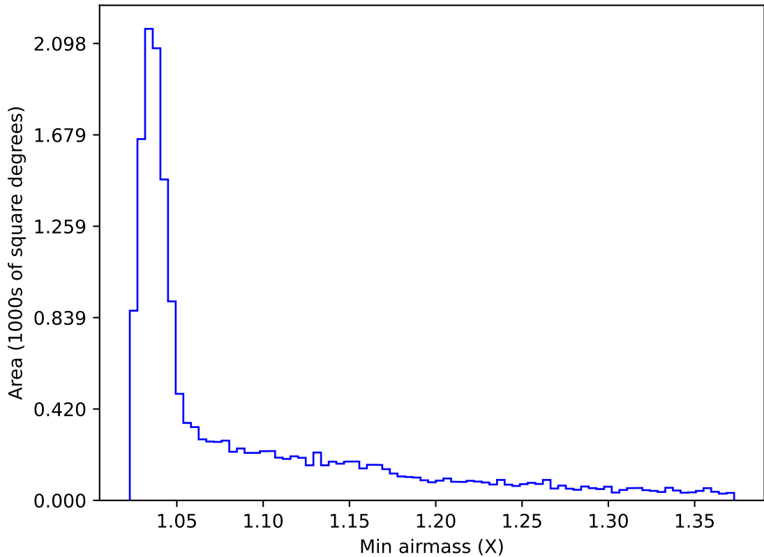
internal_u_expt60_nscale1.0v3.4_10yrs WFD g band: Min airmass
