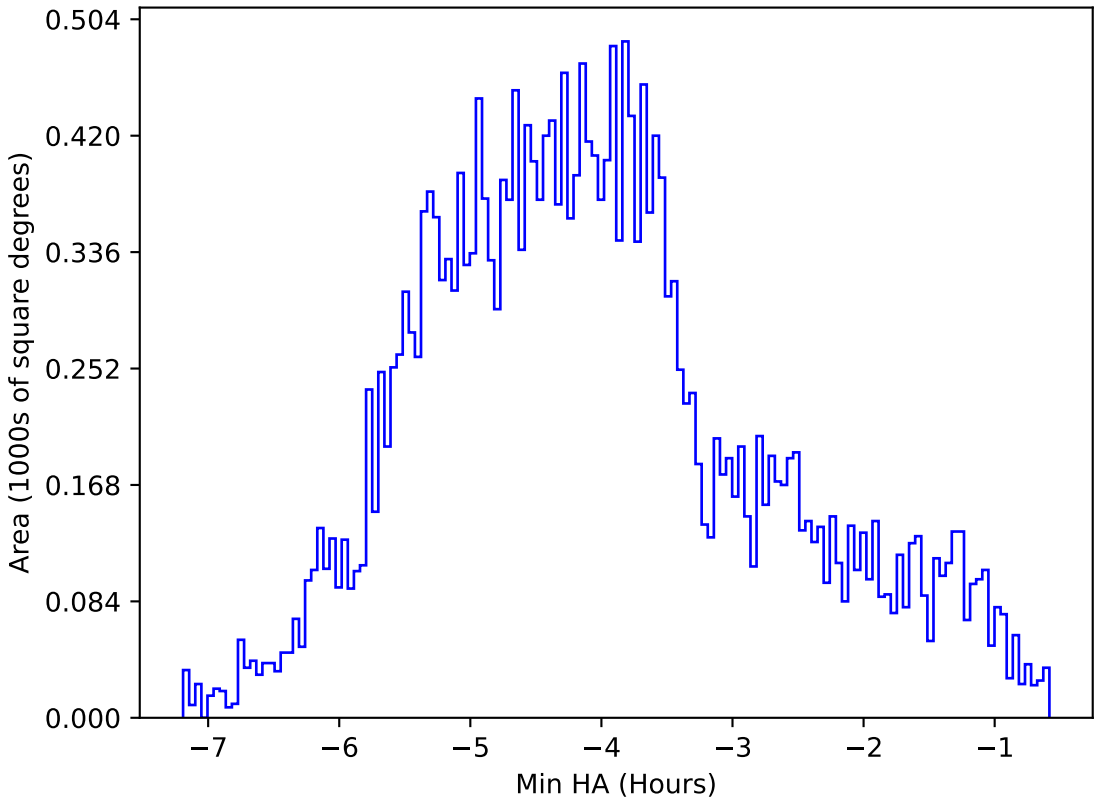
internal_u_expt60_nscale1.0v3.4_10yrs All sky z band: Min HA
