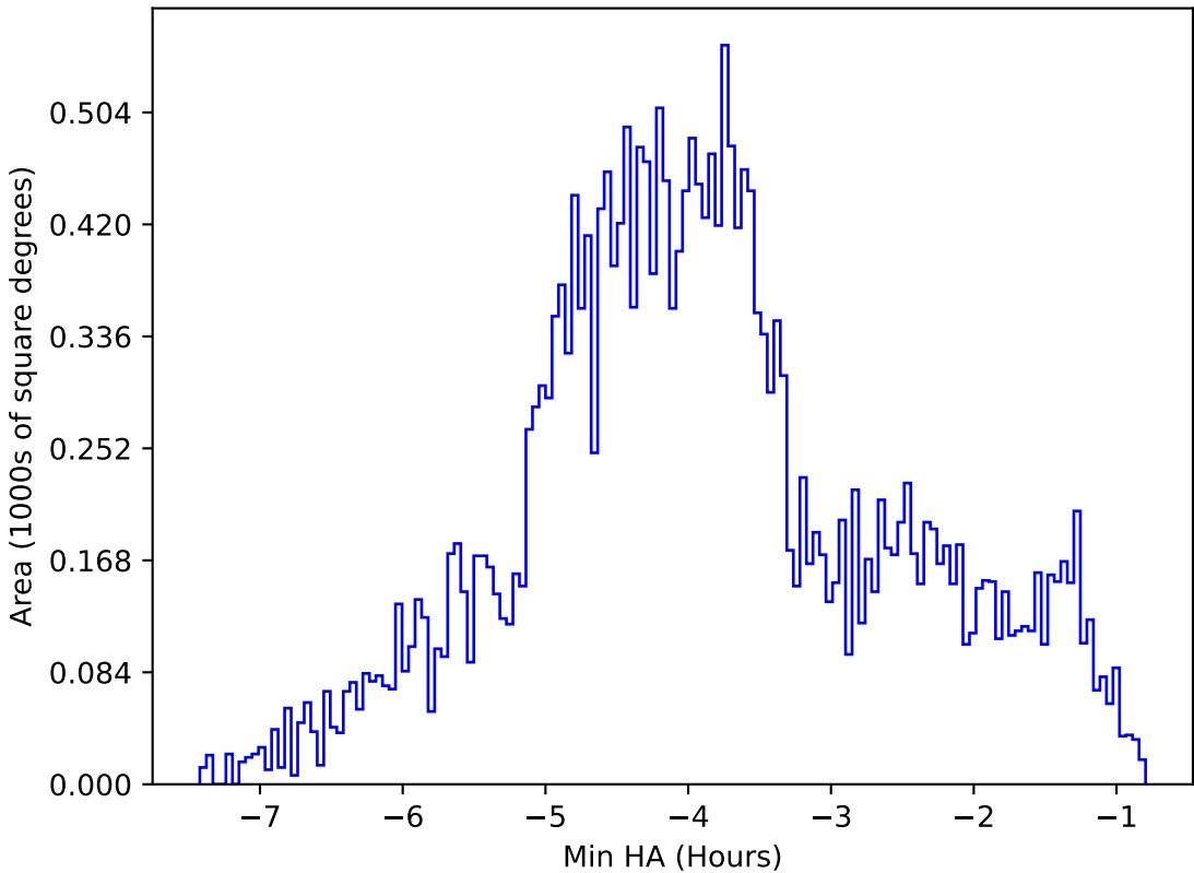
internal_u_expt60_nscale1.0v3.4_10yrs All sky g band: Min HA
